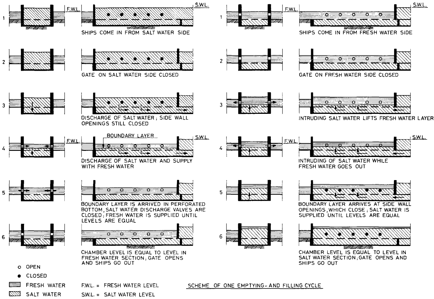
13 Figure 7. System of complete exchange of closed lock chamber.
