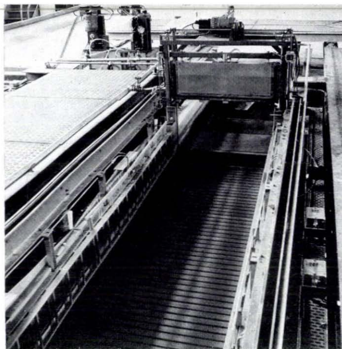
Photo 15. Overall model to a scale of 1:30, showing the perforated floor, the wall valves and the lifting gate.
