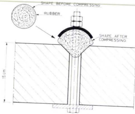
Figure 12. The joint between two beams.
