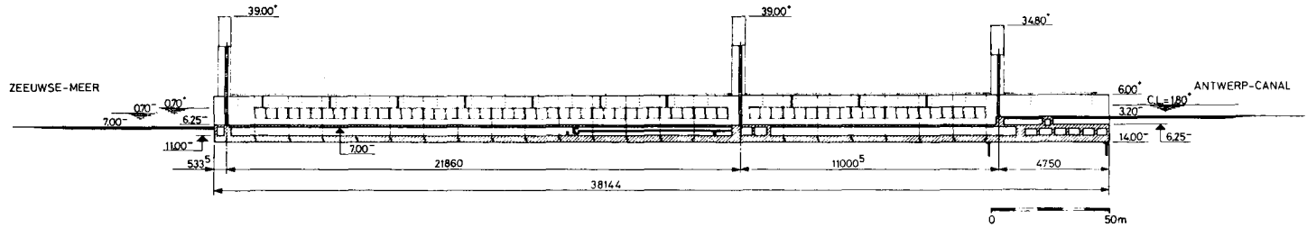
Figure 18. Longitudinal section of the lock.
