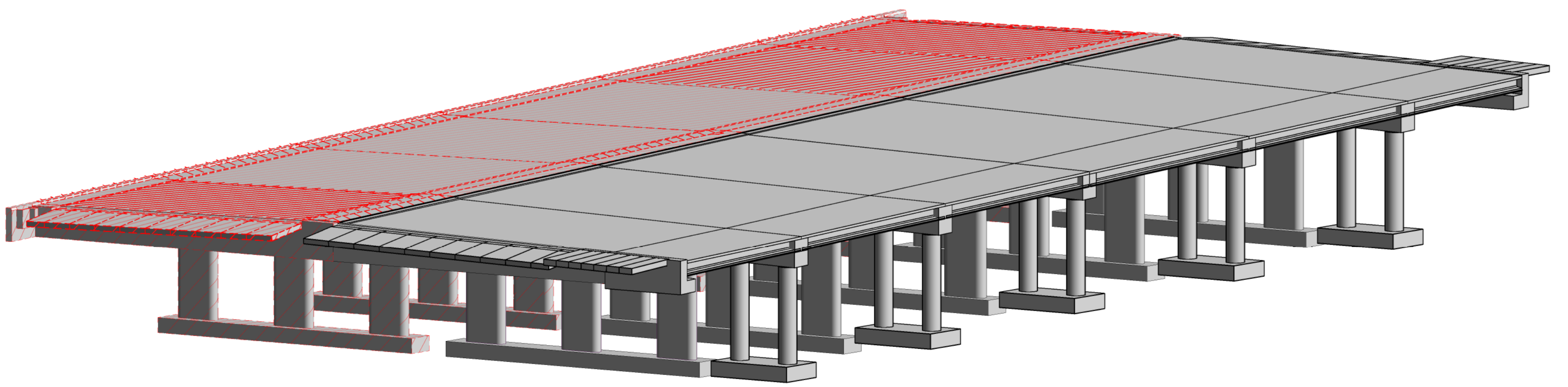
3D AANZICHT FASE 4 TE SLOPEN / 3D VIEW PHASE 4 TO DEMOLISH
